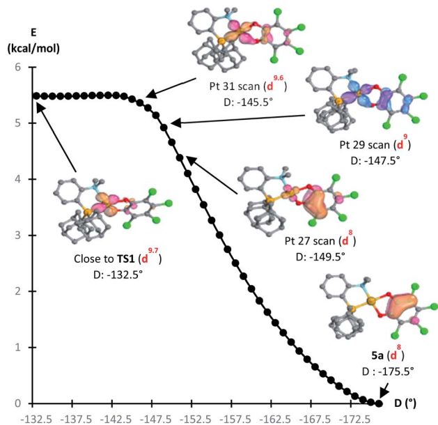
Fig. 7 Reaction path from TS1 to 5a by integrating the intrinsic reaction coordinate ( D = \text{bond dihedrals angle of } O_{cis-to-p}AuPC_{Ph} \text{ in } ^\circ ), computed at the B3PW91-D3(BJ)/SDD + f (Au), 6-31G** (C, H, N, O, P, Cl) level of theory. IBO orbitals of the Au to o -quinone electron transfer along the reaction coordinate from TS1 to 5a, showing the change from an in-plane 5d (Au) to a \pi (catecholate) orbital. Electron configuration at Au from NBO calculations.
