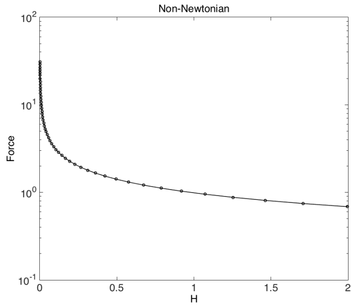
FIGURE 11 Force vs thickness: Non-Newtonian fluid
