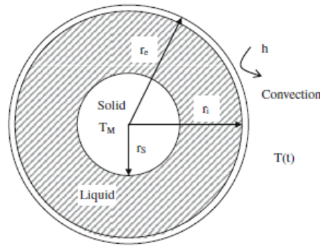
Fig. 2. Melting inside a spherical capsule. Adapted from [9].
